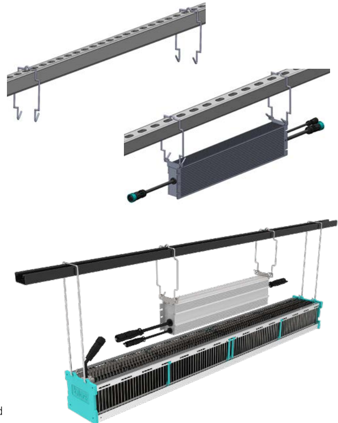
Unistrut Channel-Side Down
